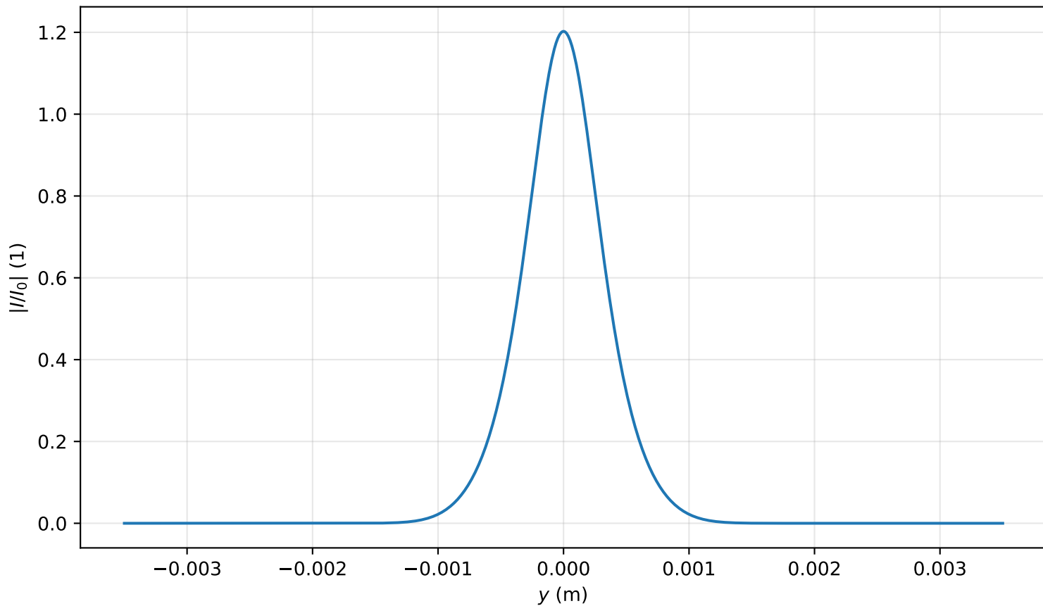
Intensity profile I(x=0, y, z=0.716)/I_0 , P_{in}=0.8P_{cr} , artificial time
